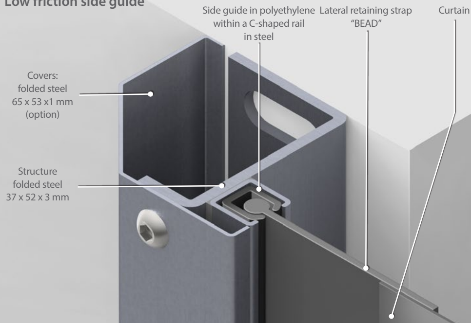
Low friction side guide
